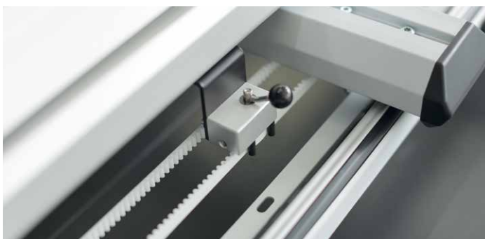
One-touch quick belt release system
